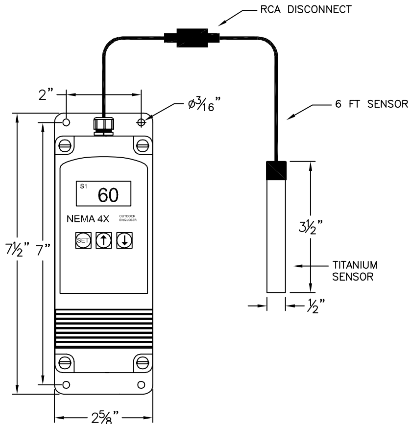
TRSN AND TRDN CONTROLLER
